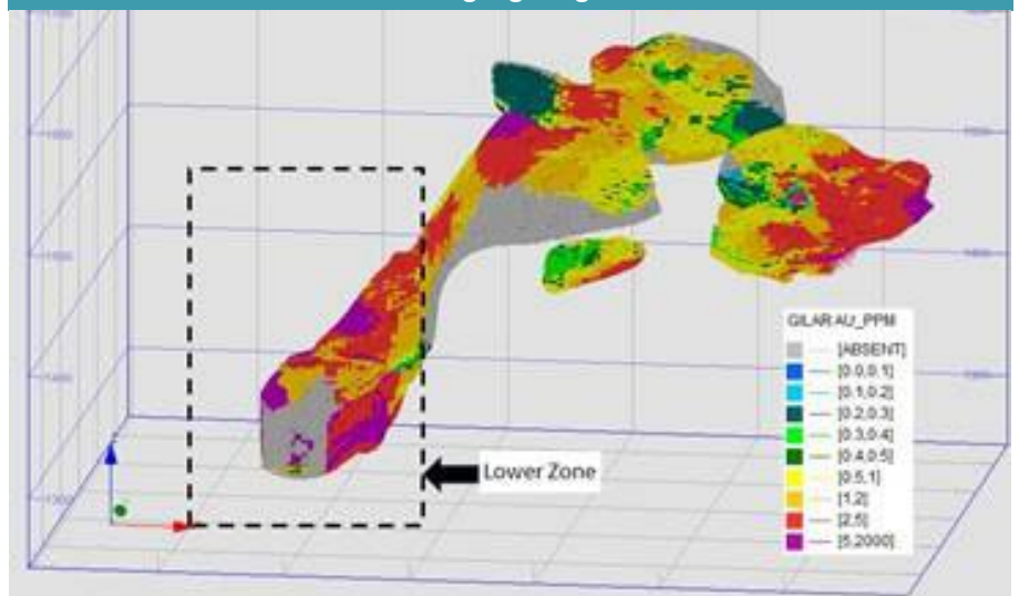
Gilar mineralisation block model highlighting lower zone
